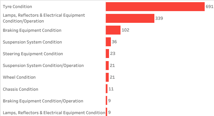
Top 10 Dangerous Defects detected Roadside(RW) 2023
