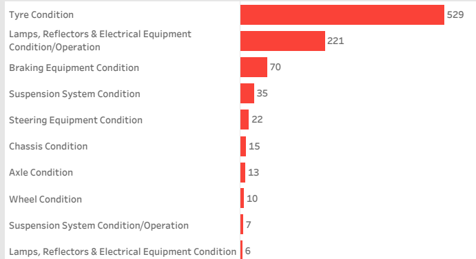
Top 10 Dangerous Defects detected Roadside (RW) 2024
